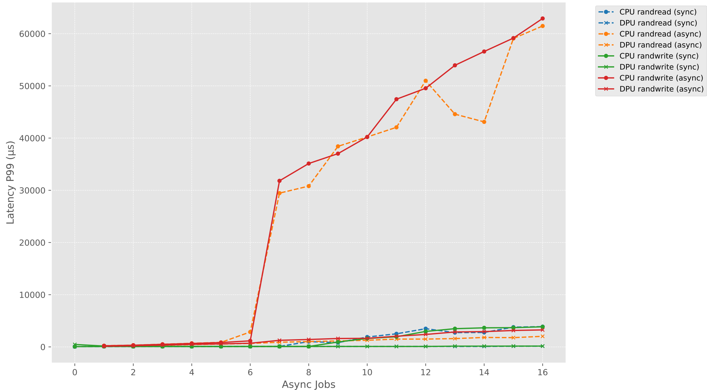
Latency P99 vs Async Jobs (sync1_asyncN) - RAND (CPU vs DPU)
